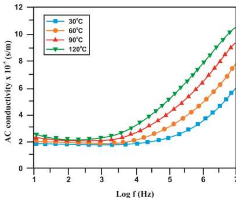
Fig.10 Variation of AC conductivity with frequency
